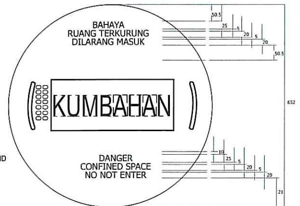
Detail 2 & 3 : Embossed Design
