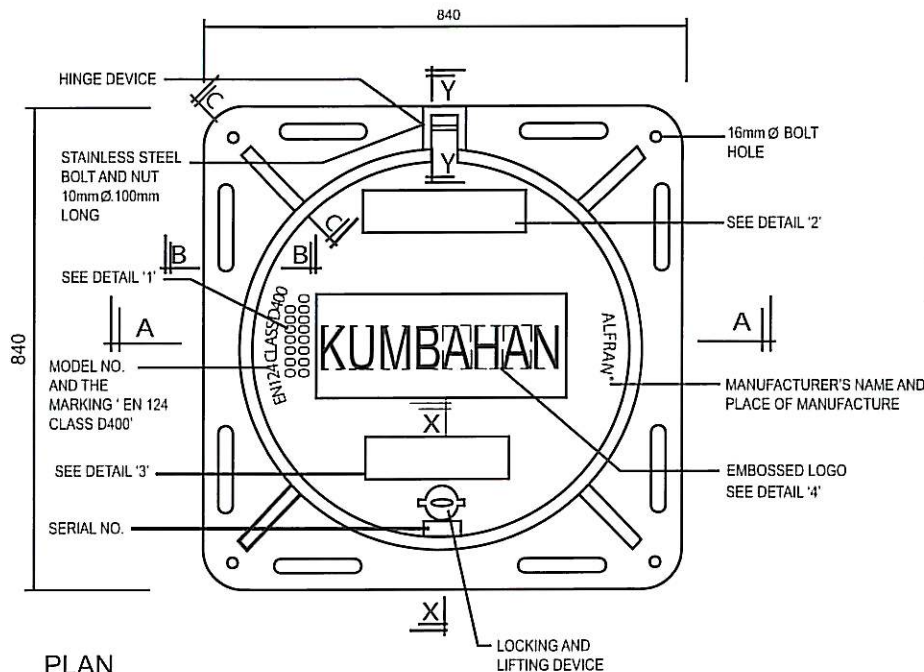
PLAN TYPICAL DETAILS OF HEAVY DUTY D.I. MANHOLE COVER AND FRAME
